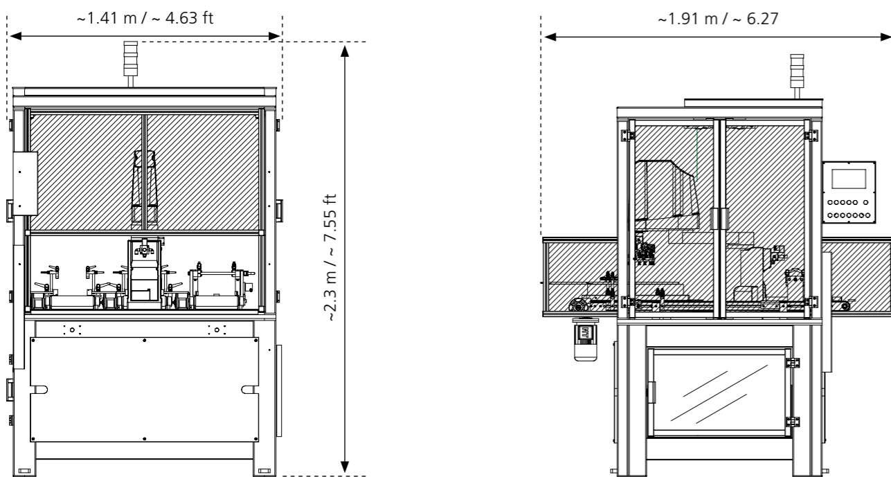
Misure macchina Machine measure
