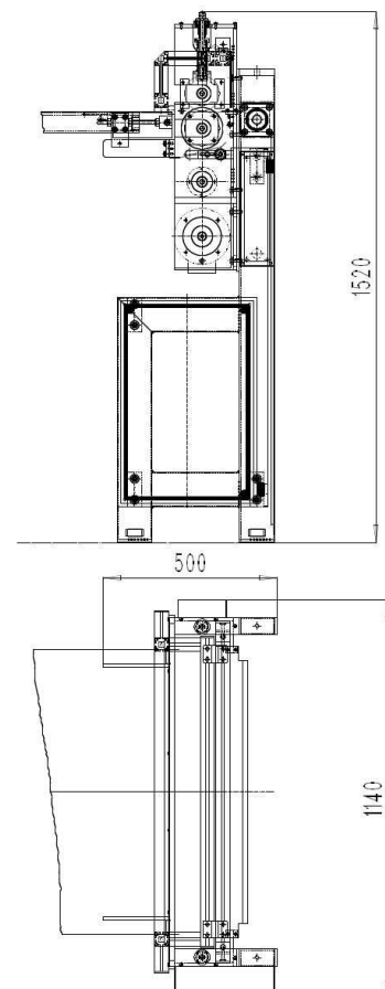
MC19 Layout e Ingomri Layout and Overall Dimensions
